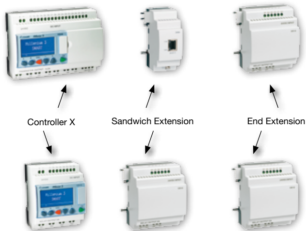
Fig. 4 – Extension units can provide digital/analog I/O, Modbus/Ethernet communication
